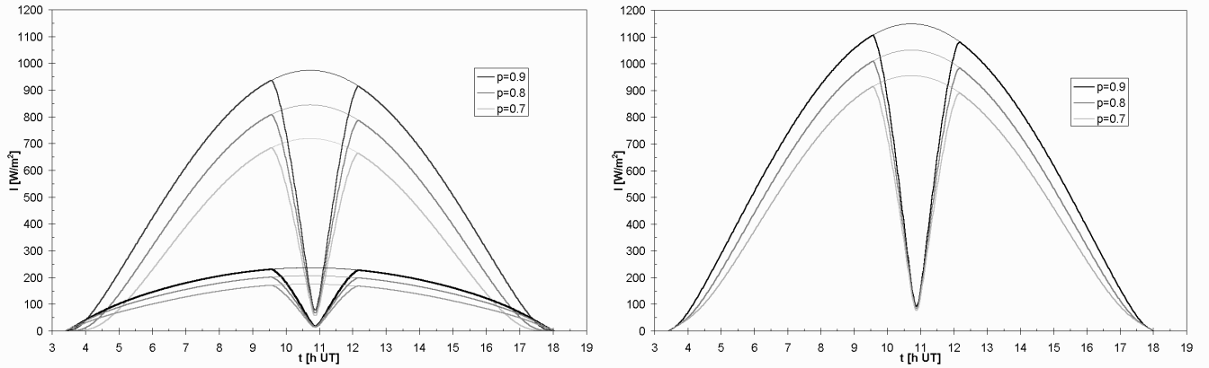
Fig.4. Modelled solar direct, scattered (left) and total (right) radiation flux in Szczawnica at the day of eclipse.
