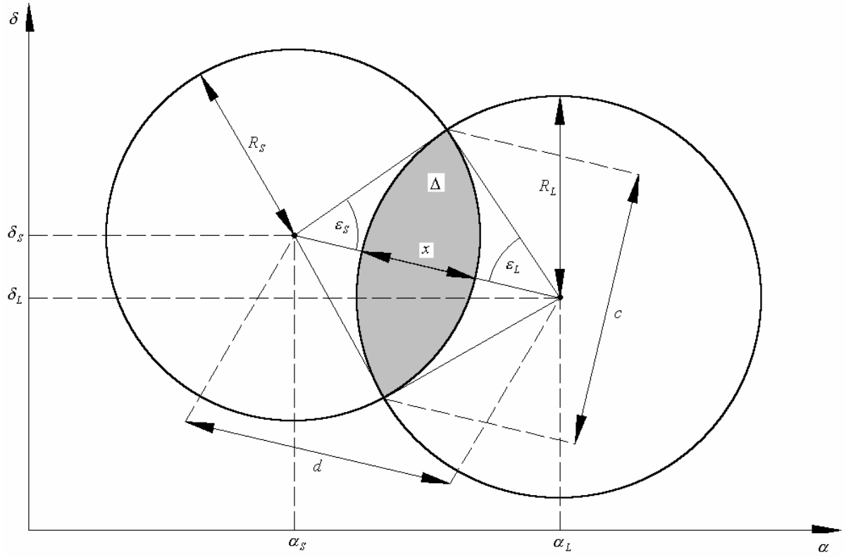
Fig.1. Geometric model of the solar eclipse.
