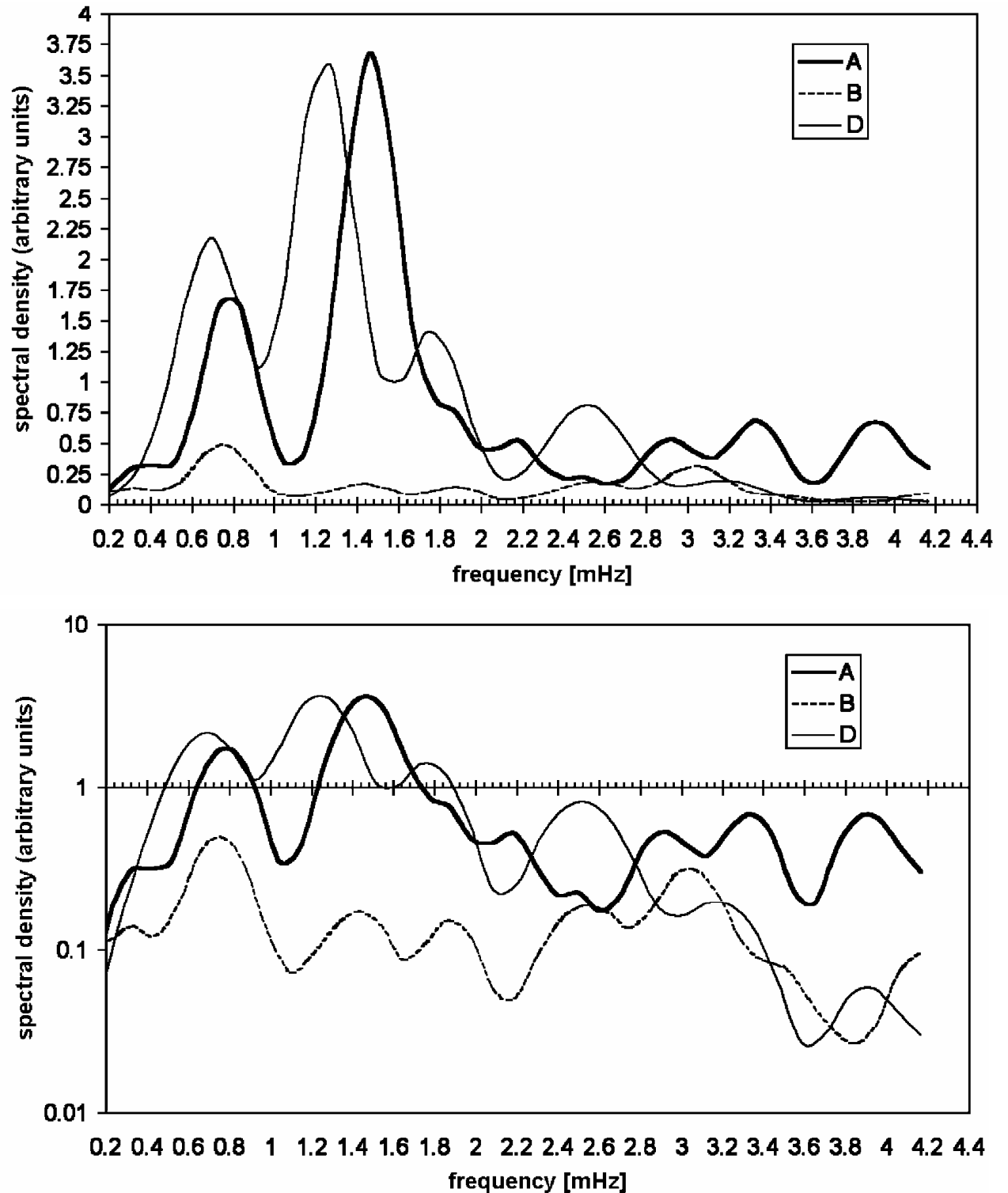
Fig. 12. FFT spectra of thermal fluctuations for ranges A, B and D.
