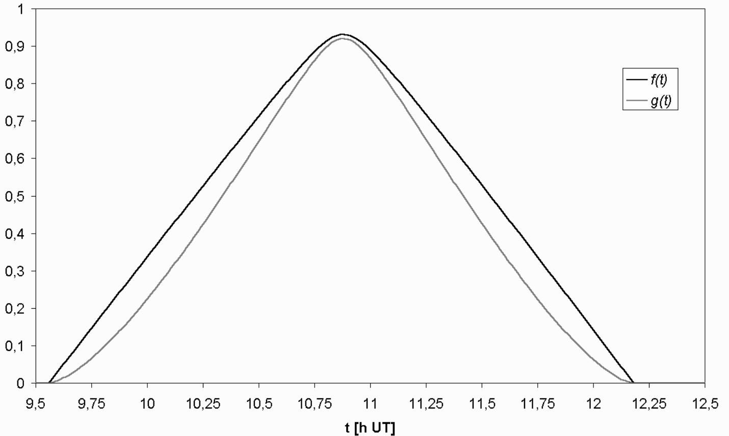
Fig.2. Astrometric parameters during the 11 th August 1999 eclipse in Szczawnica.
