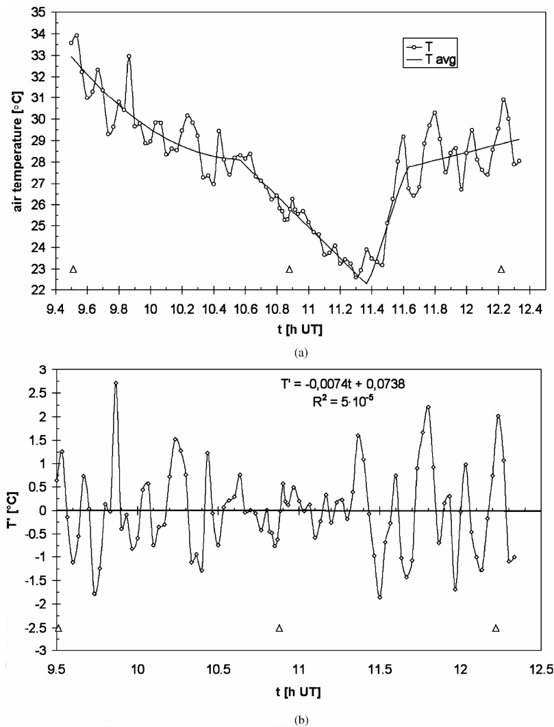
Fig. 10. (a) The measured temperature towards the fitted model of mean temperature.
