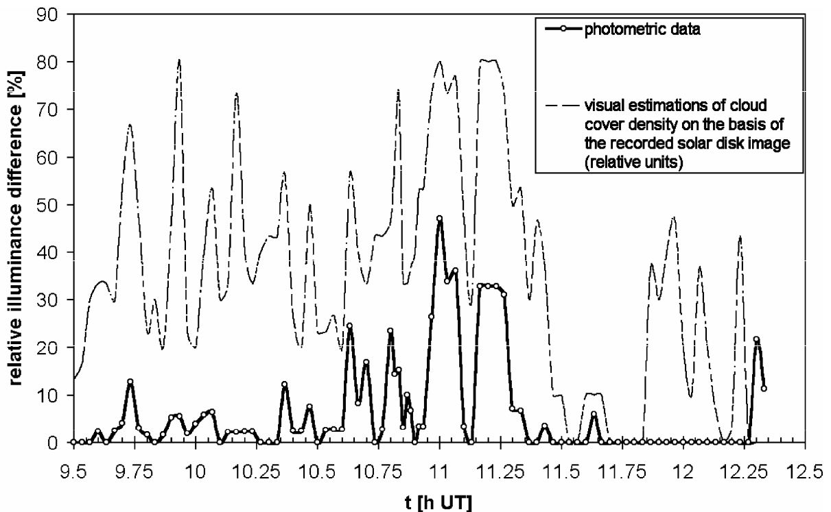
Fig. 7. Relative difference in both sensors' illumination, being the measure of the cloud cover.
